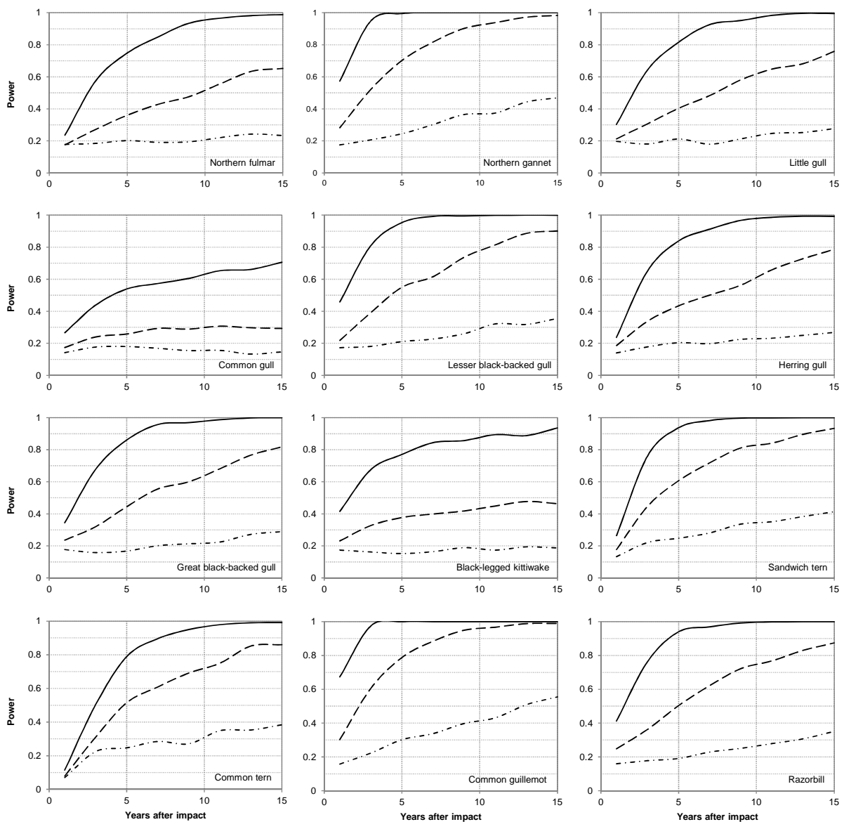
Figure 37. Power results for 12 seabird species for an impact study with a monitoring intensity of one survey of 10 km 2 per month per area, and 5 years of reference monitoring (significance level = 0.10).
