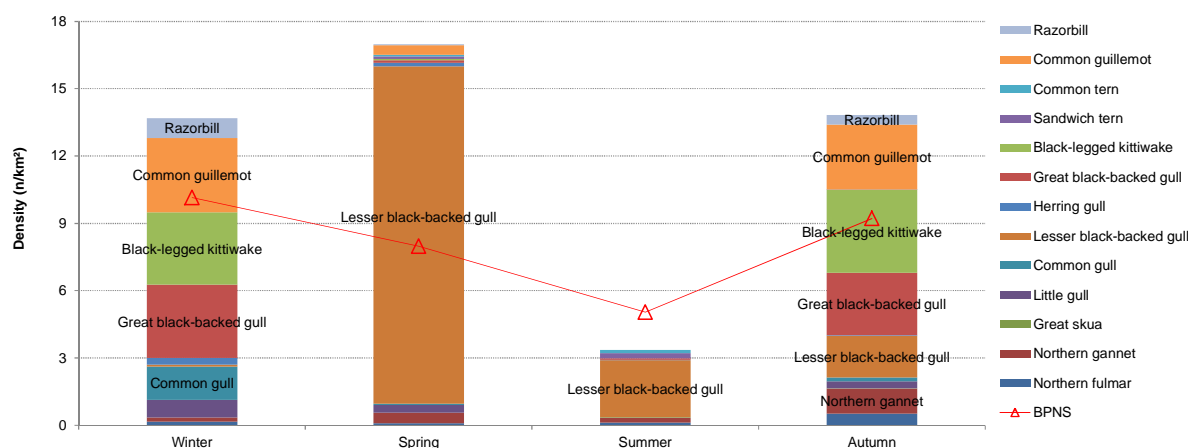
Figure 19. Seasonal densities of seabirds in the impact area at the Thorntonbank before wind farm construction (<04/2008), with indication of the cumulative seabird density at the BPNS.
