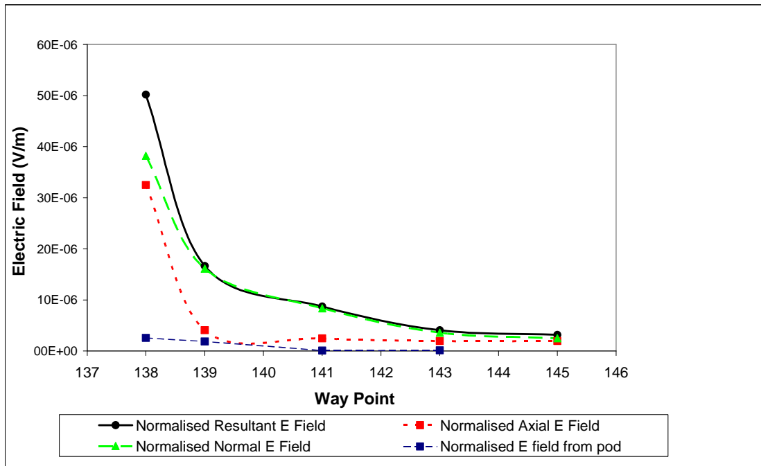
Figure 32. Electric field variation along western cable route.
