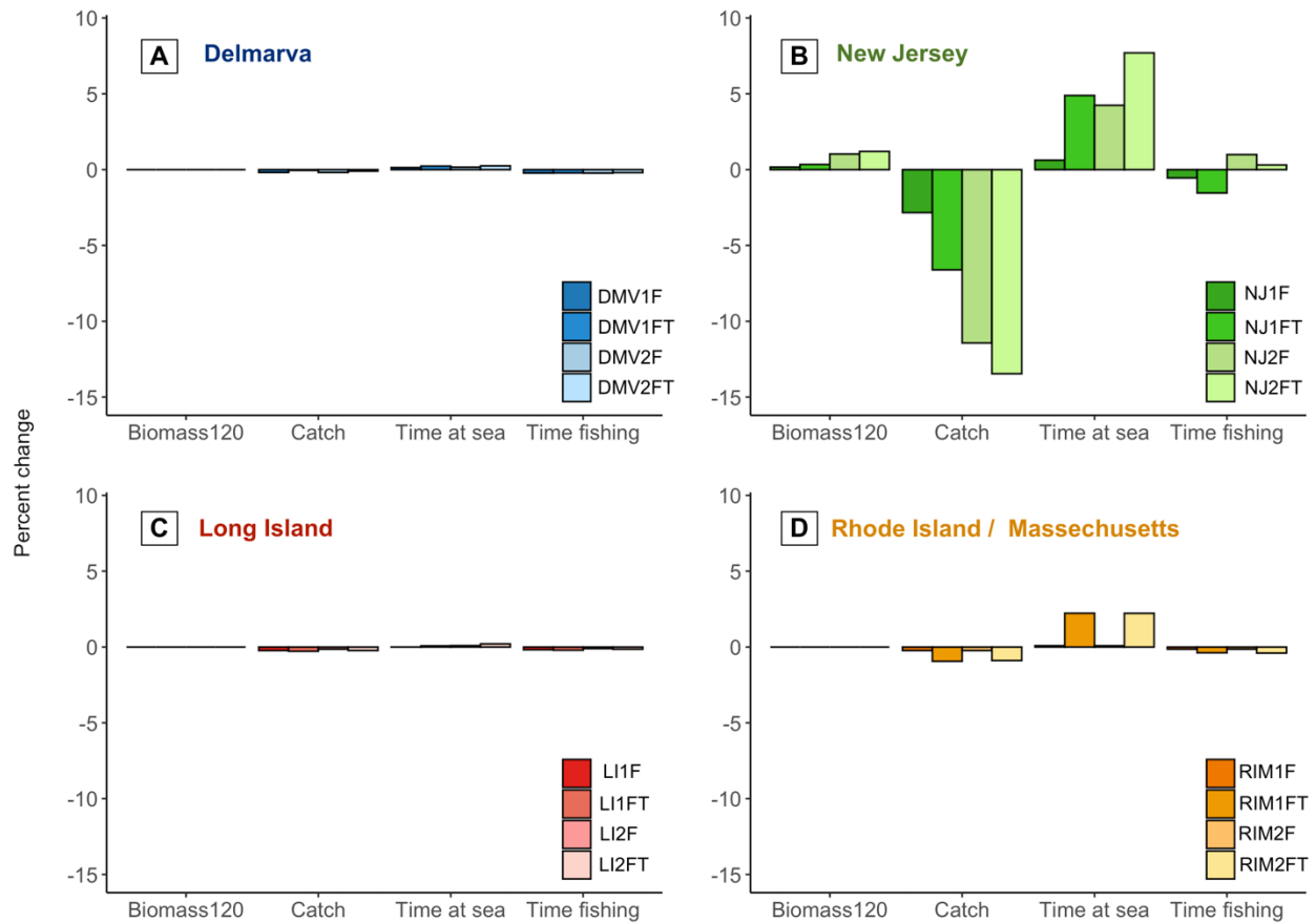
Figure 15: Change in biology and fishery behavior for regional wind area simulation scenarios.
