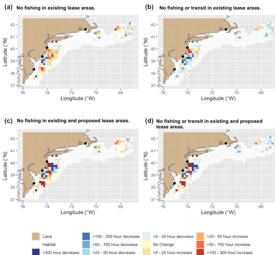
Figure 12: Simulated fishery effort displacement for cumulative impact simulation scenarios. Simulated Atlantic surfclam fishing effort displacement, indicated by the change in the average number of hours fished per model grid cell per year, for scenarios that allow (a) transit but no fishing in existing lease areas (Cum1F), (b) neither transit nor fishing in existing lease areas (Cum1FT), (c) transit but no fishing in existing and proposed lease areas (Cum2F), (d) neither transit nor fishing in existing and proposed lease areas (Cum2FT). Fishing effort displacement in each model grid cell was calculated for each simulation scenario relative to the average annual hours fished in that grid cell with no transit or fishing restrictions (StatusQuo, reference simulation). A decrease (increase) in average effort for a model grid cell under a particular scenario indicates behavioral restrictions led to less (more) time fishing in that area.
