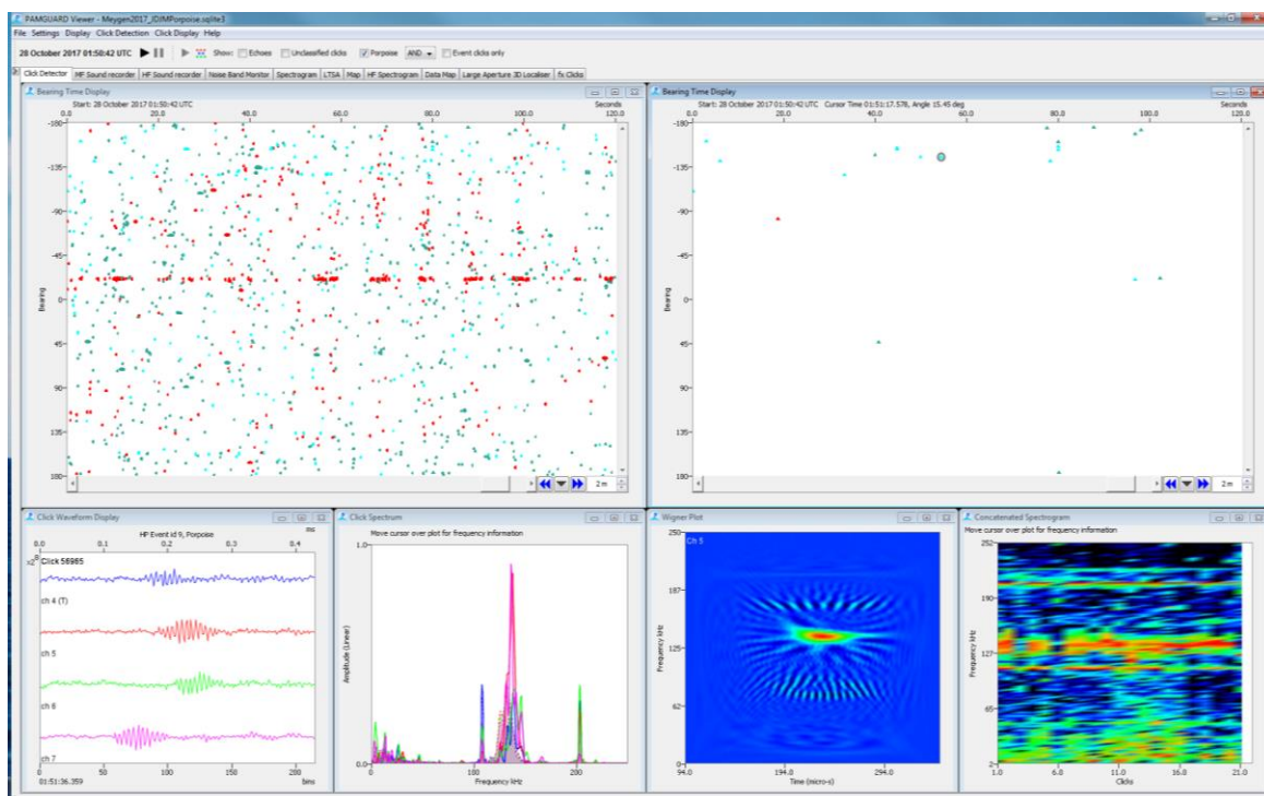
Figure 11. PAMGuard analysis display. The two larger top windows show the bearing and amplitude of clicks plotted against time over a 2 minute period. The smaller lower plots show the waveform, power spectrum and Wigner plot of individual clicks and a concatenated spectrum of all clicks manually assigned to an “event”.
