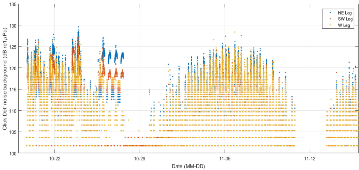
Figure 4. Data showing noise in the click detector frequency band from each hydrophone cluster. There are changes by up to 20dB over a tidal cycle and between neap-spring tides. Such changes significantly impact the range at which harbour porpoises and dolphins can be detected.
