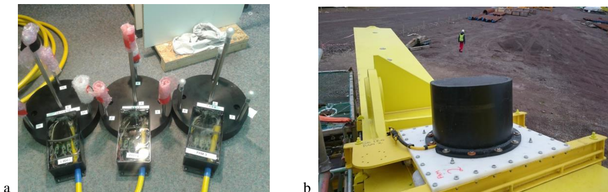
Figure 10. a. Assembled hydrophone clusters with potted hydrophones and data cables, b. the hydrophone cowling and mounting plate attached to a leg of the TSS.
