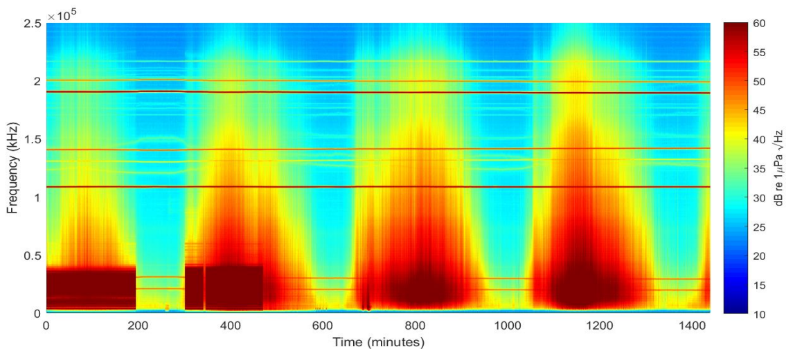
Figure 5. A long term spectral average of four tidal cycles. In the first two cycles the turbine is operational and high levels of low frequency noise below 50 kHz is clearly visible. In the last two tidal cycles the turbine is not operational and noise in the lower frequency band is reduced.
