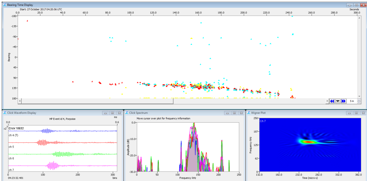
Figure 2. PAMGuard display during a porpoise encounter on 27 October. The top panel of the display shows bearings to clicks from each hydrophone cluster (each cluster being represented by a different colour). The bottom panels show the waveform, spectrum and Wigner (time-frequency) plot for a single selected click.
