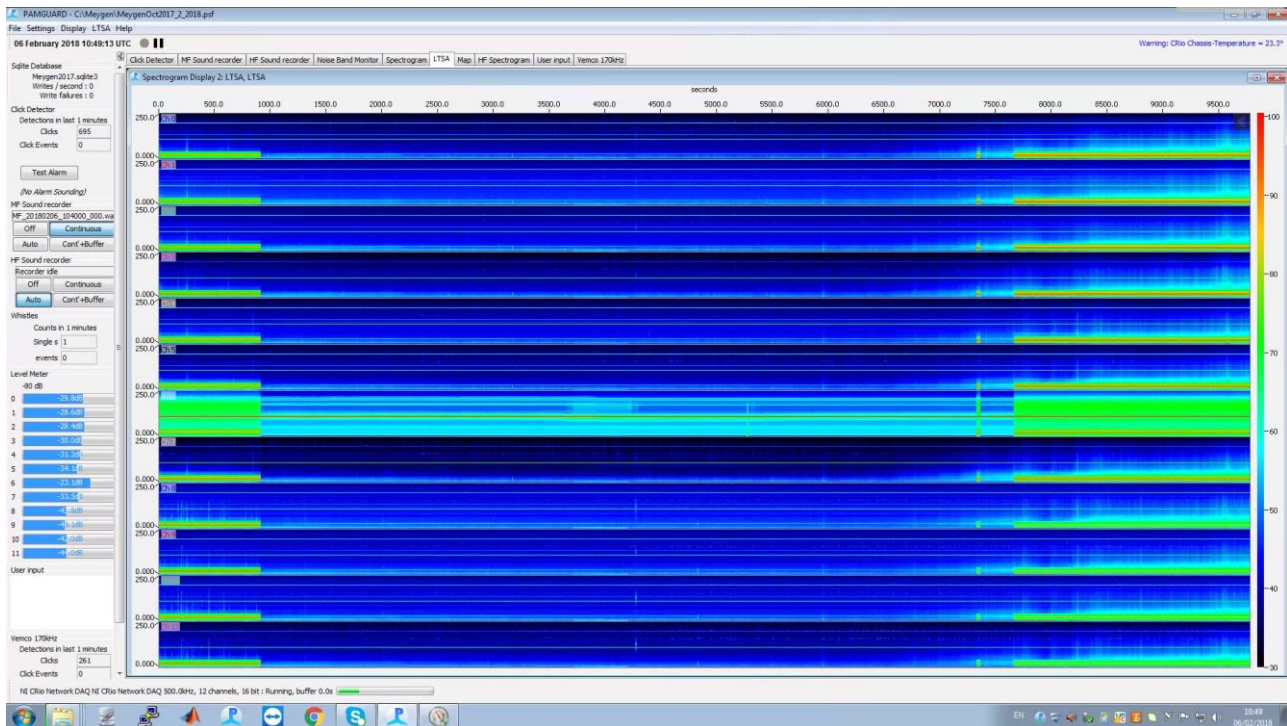
Figure 1. Screenshot of the PAMGuard data collection software showing a long term (approximately 3 hours) spectral average output from each of the 12 hydrophones. The spectral average is colour coded to show periods of relatively low (blue) to high (red) noise. Periods of tidal flow and turbine operating are apparent at the start and end of the display with a relatively low noise period in the middle. Note that a constant tonal noise at a frequency of 108 kHz is apparent on hydrophone 7.
