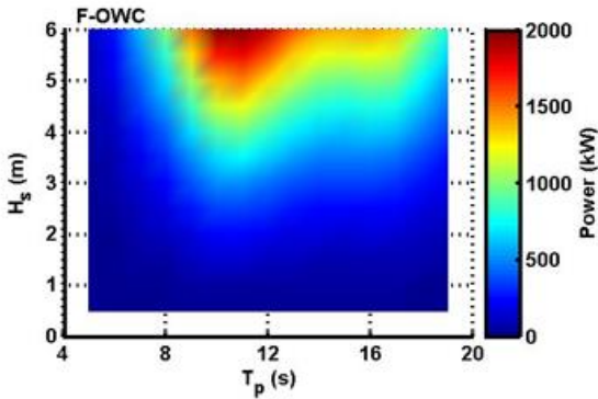
FIGURE 1. POWER MATRICES COMPUTED FOR THE F-OWC WEC DEVICE AS A FUNCTION OF SIGNIFICANT WAVE HEIGHT AND PEAK WAVE PERIOD.
