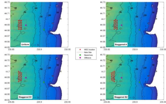
FIGURE 2. ARRAY CONFIGURATIONS AND LOCATION OF OFFSHORE AND NEARSHORE COMPARISONS
