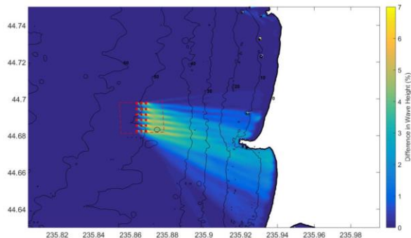
FIGURE 3. PERCENT DIFFERENCE IN SIGNIFICANT WAVE HEIGHT FOR THE UNIFORM CONFIGURATION.
