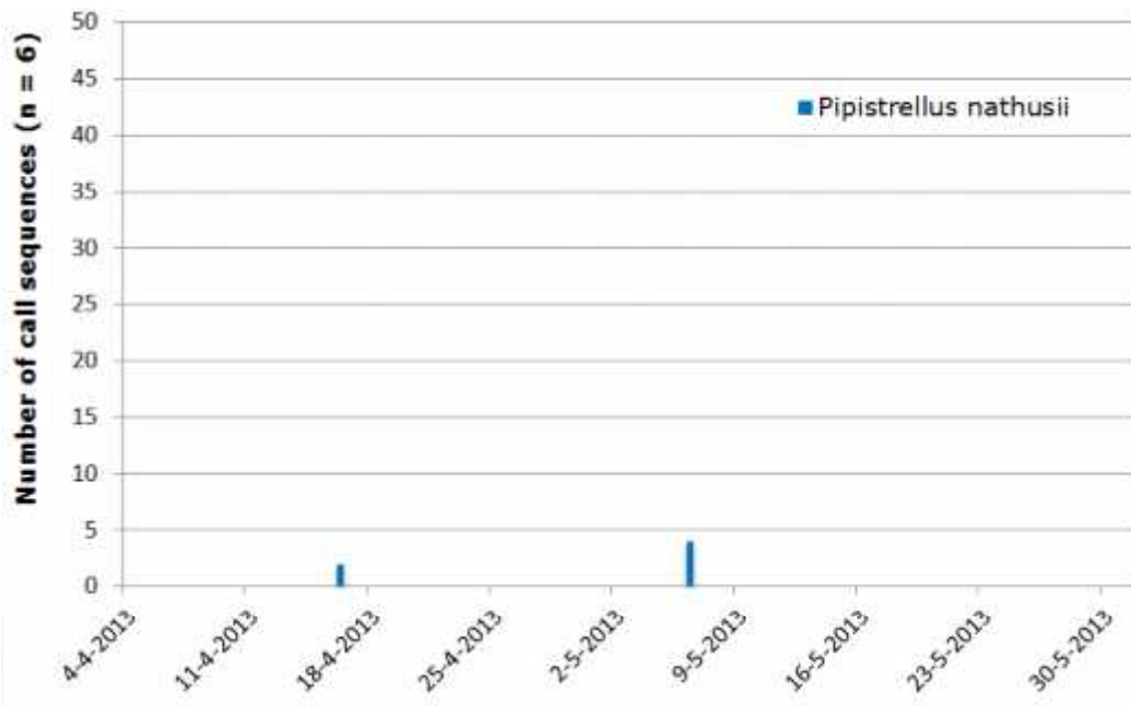
Figure 6. Number of call sequences per night at OWEZ spring 2013.
