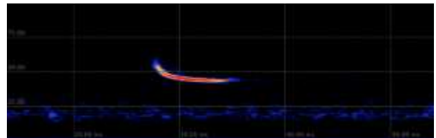
Figure 3: Spectrogram of Common pipistrelle 25 August 2013 PAWP
