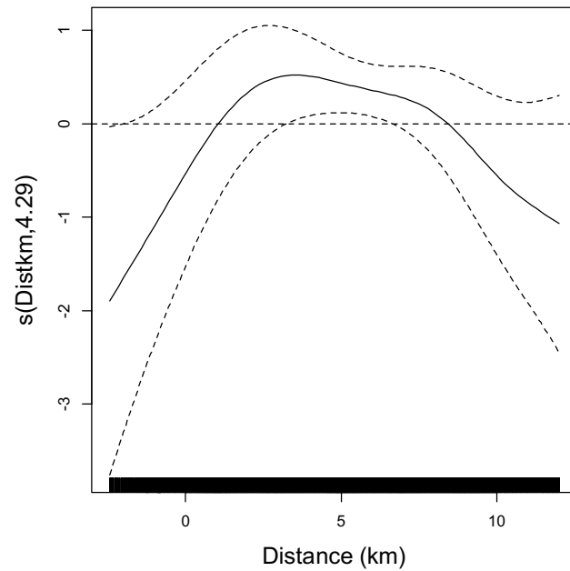
Figure 10. Distance smoother for the HornsRevI data.
