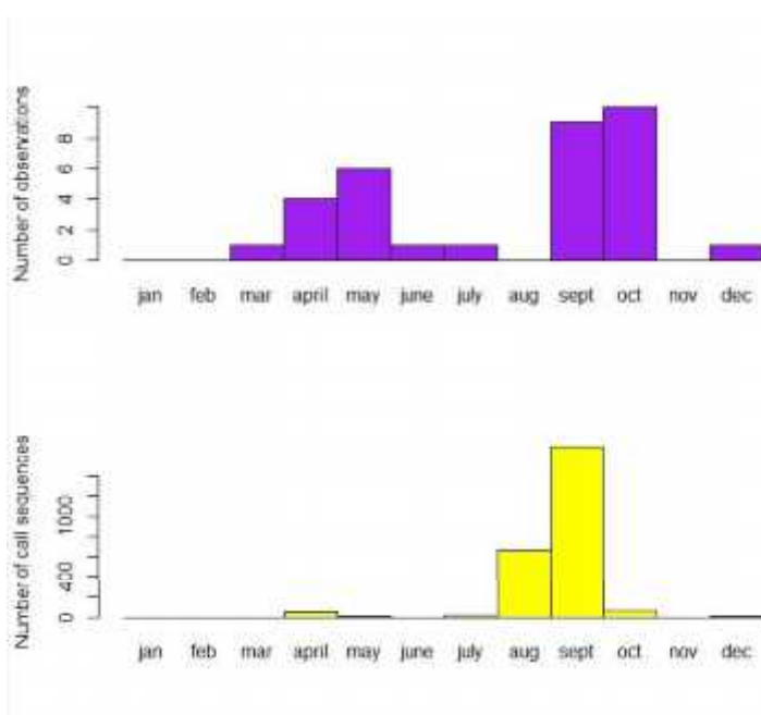
Figure 4.55. Temporal occurrence of Nathusius' Pipistrelle.
