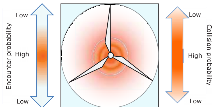
Figure 4.44. Representation of variation in encounter probability with height and collision risk throughout the rotor-swept area. Combined, these two factors result in a low overall collision risk at the altitudinal extremities of the rotors.
