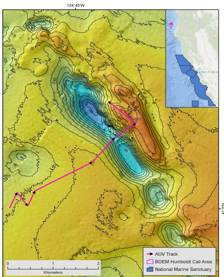
Figure 2.2. Location of large ridge feature in the HWEA (image from: NOAA, BOEM, and USGS 2019).
