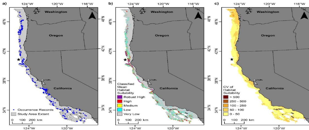
Figure 3.3. Predicted habitat suitability for the soft coral Heteropolypus ritteri (Alcyonacea, Alcyoniidae). (a) Records of H. ritteri occurrence from the NOAA National Database for Deep-Sea Corals and Sponges within the study area offshore to 1,200 m depth; (b) classified mean habitat suitability for H. ritteri ; and (c) coefficient of variation of the mean habitat suitability for H. ritteri . (Figure reproduced from Poti et al. 2020; star indicates general location of the Humboldt Wind Energy Area)
