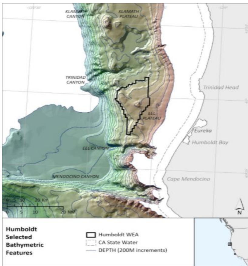
Figure 1.3. Selected bathymetric features within and around the HWEA.
