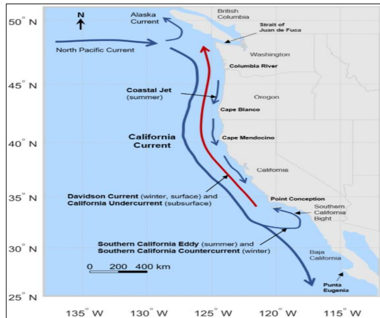
Figure 1.2. Schematic of the California Current System
