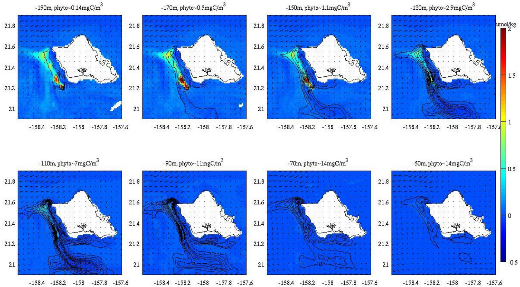
Figure 71. Nitrate perturbation ( \mu\text{mol/kg} ) due to the RevX 3x100MW OTEC plant, and contour lines of the resultant diatom perturbation (black lines) drawn at intervals of 0.5 mgC/m 3 . June 24 th , 2010 at 16:40 Hawaiian Standard Time.
