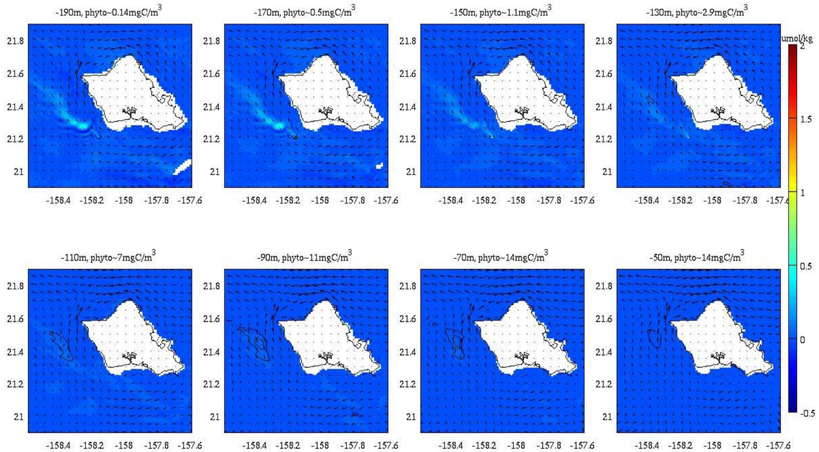
Figure 88. Nitrate perturbation ( \mu\text{mol/kg} ) due to the RevX 100MW 8x95m OTEC plant, and contour lines of the resultant pico-phytoplankton perturbation (black lines) drawn at intervals of 0.5 \text{ mgC/m}^3 . June 3 rd , 2010 at 16:40 Hawaii Standard Time.
