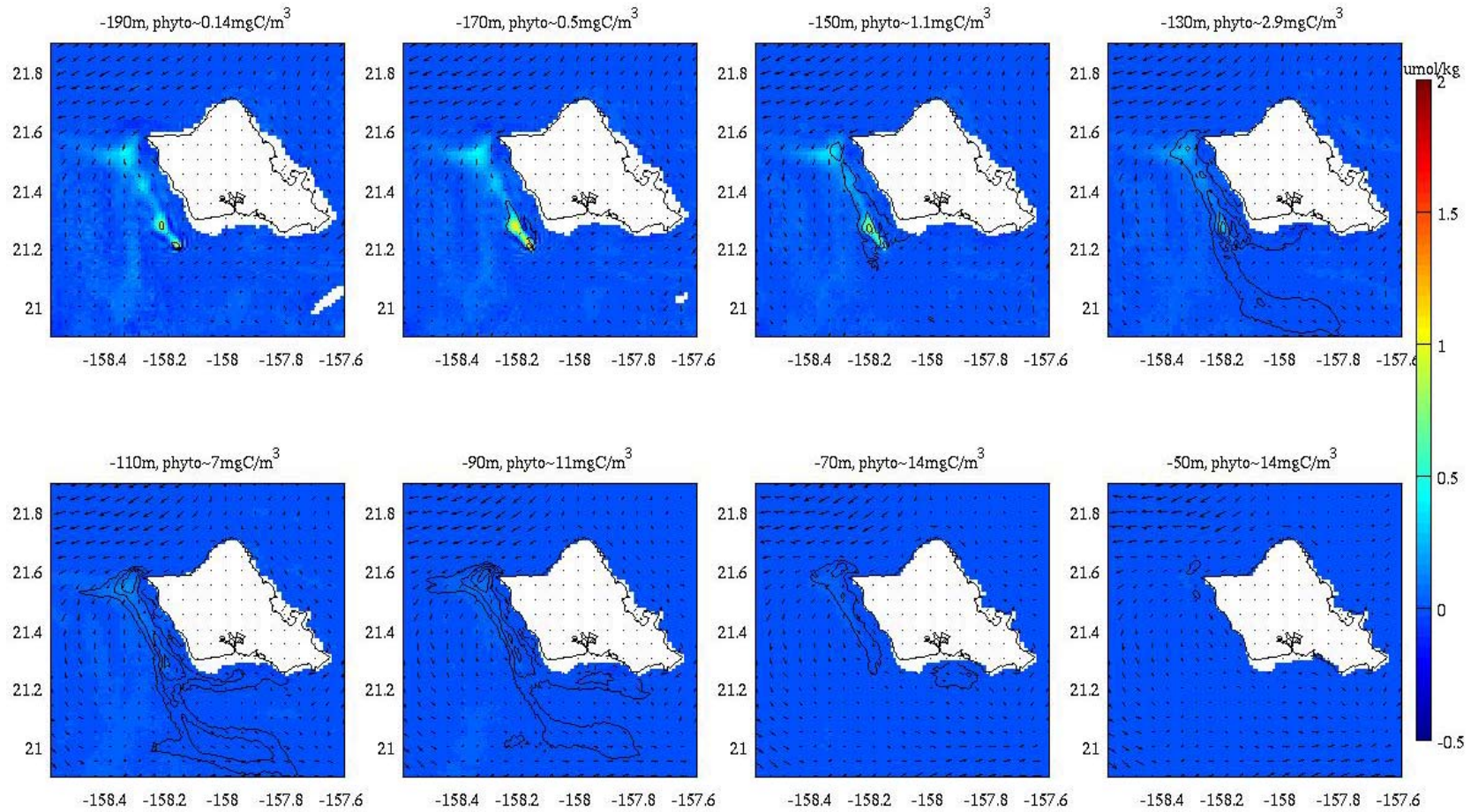
Figure 55. Nitrate perturbation ( \mu\text{mol/kg} ) due to the RevX 100MW OTEC plant, and contour lines of the resultant diatom perturbation (black lines) drawn at intervals of 0.5 \text{ mgC/m}^3 . June 24 th , 2010 at 16:40 Hawaii Standard Time.
