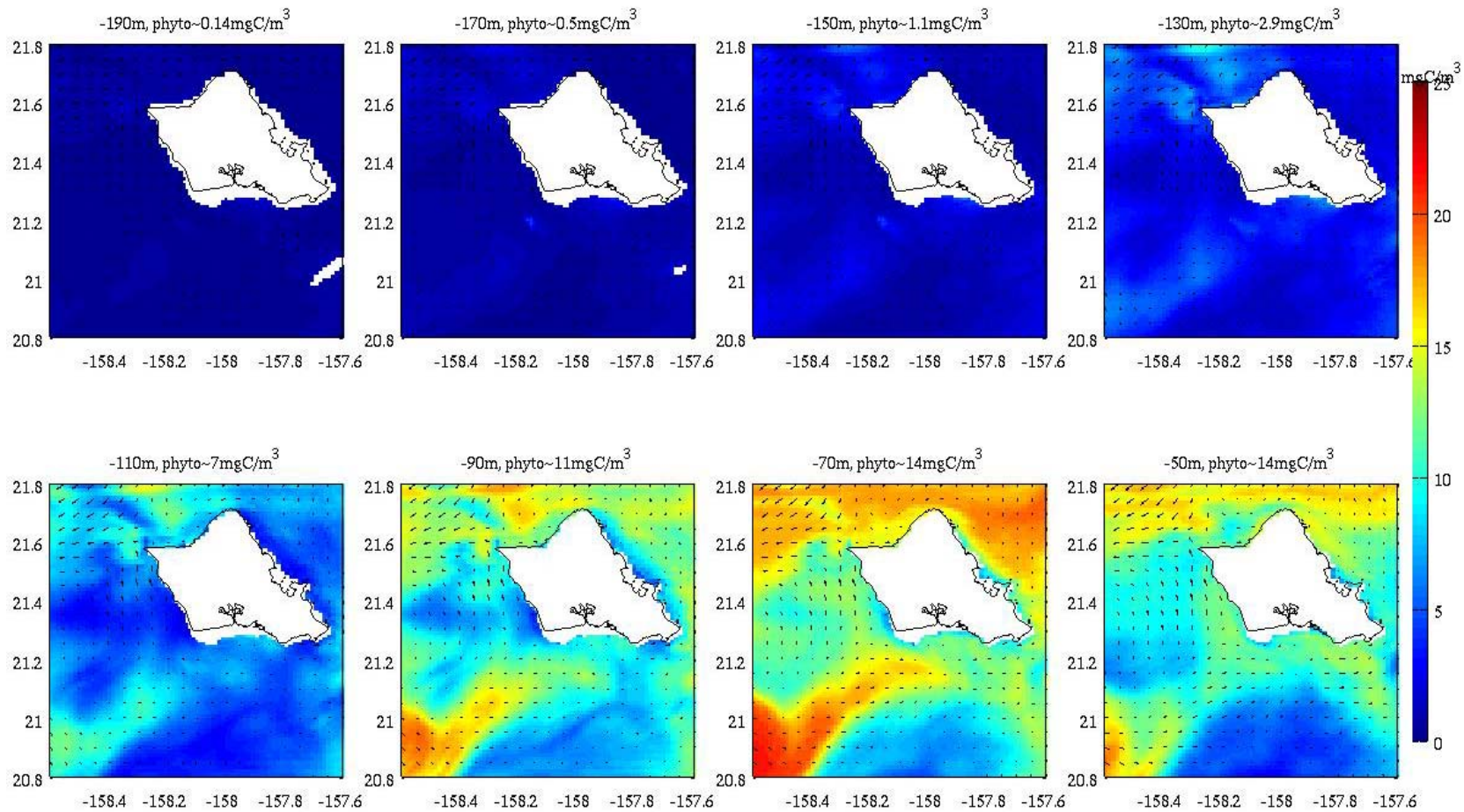
Figure 58. Pico-phytoplankton biomass (prochlorococcus, synechococcus, etc.) in \text{mgC/m}^3 from the RevX 3x100MW OTEC simulation. Figures show the plan view at 190, 170, 150, 130, 110, 90, 70, and 50 meter depths at at June 17 th at 16:40 Hawaii Standard Time.
