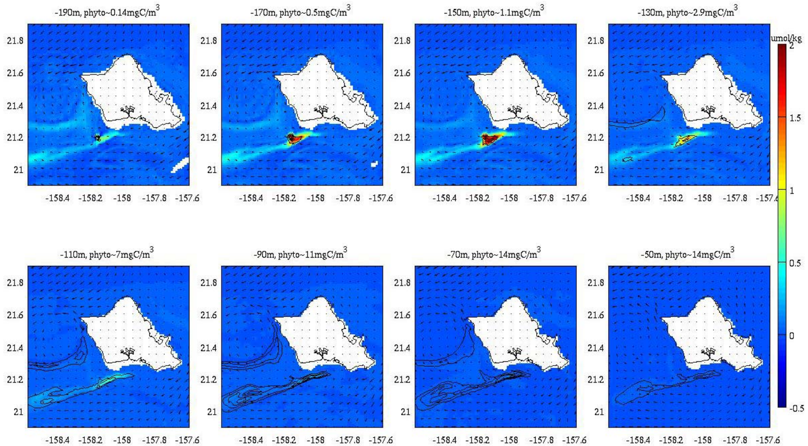
Figure 61. Nitrate perturbation (umol/kg) due to the RevX 3x100MW OTEC plant, and contour lines of the resultant pico-phytoplankton perturbation (black lines) drawn at intervals of 0.5 mgC/m 3 . June 10 th , 2010 at 16:40 Hawaii Standard Time.
