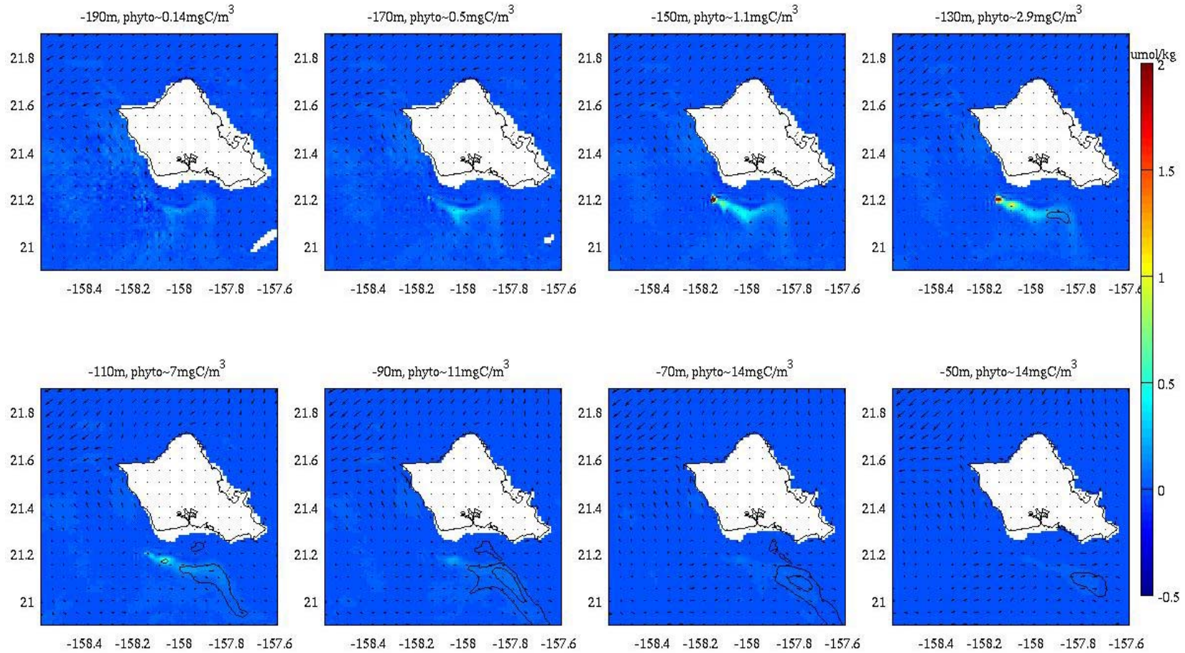
Figure 86. Nitrate perturbation ( \text{umol/kg} ) due to the RevX 100MW 8x70m OTEC plant, and contour lines of the resultant diatom perturbation (black lines) drawn at intervals of 0.5 \text{ mgC/m}^3 . June 17 th , 2012 at 16:40 Hawaii Standard Time.
