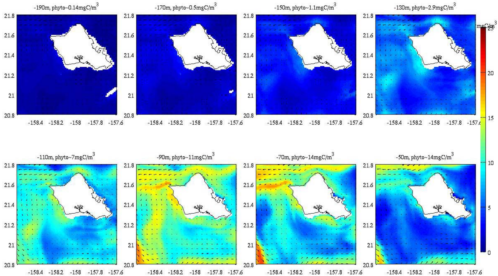
Figure 43. Pico-phytoplankton biomass (prochlorococcus, synechococcus, etc.) in \text{mgC}/\text{m}^3 from the RevX 100MW OTEC simulation. Figures show the plan view at 190, 170, 150, 130, 110, 90, 70, and 50 meter depths at June 24 th at 16:40 Hawaii Standard Time.
