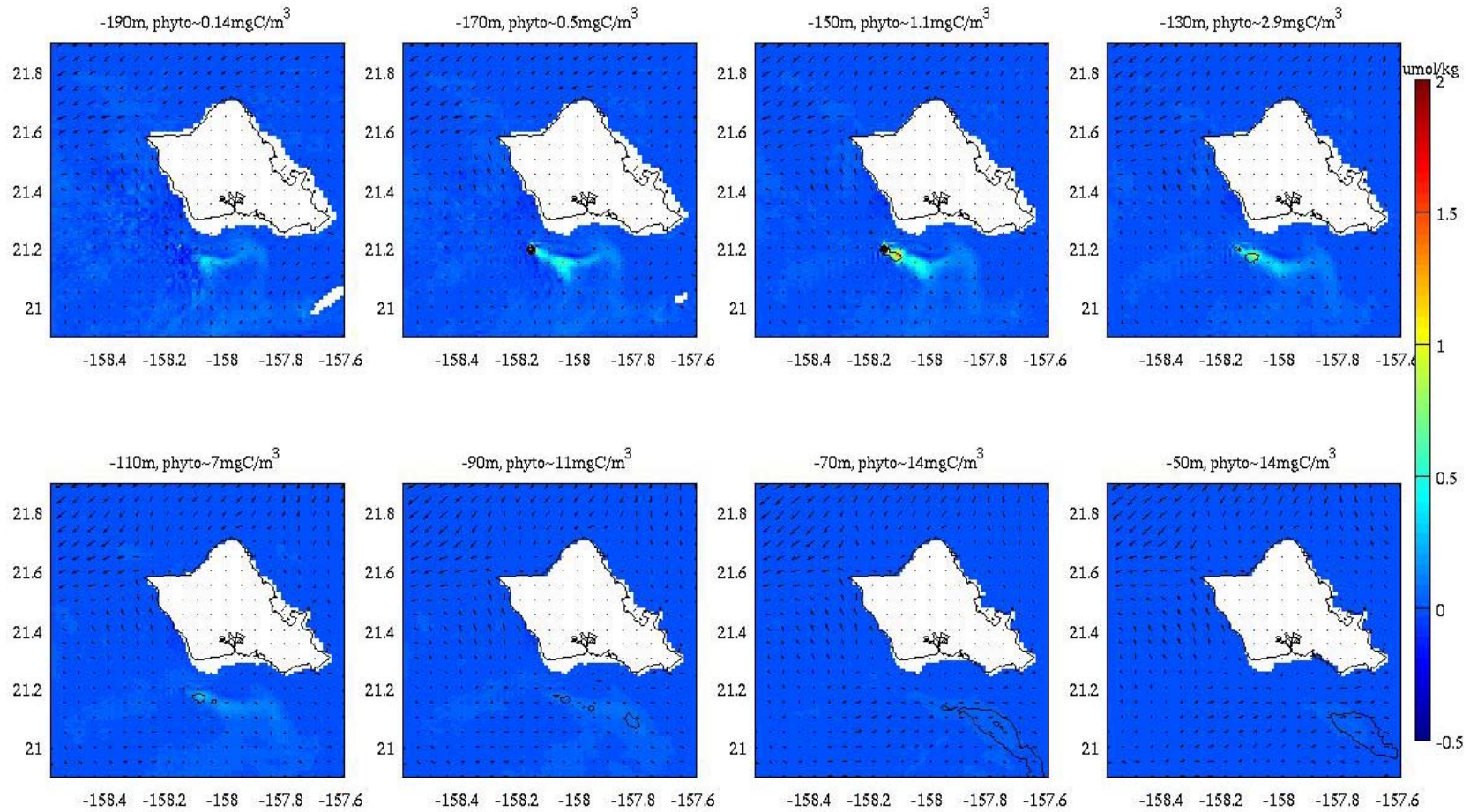
Figure 46. Nitrate perturbation ( \mu\text{mol/kg} ) due to the RevX 100MW OTEC plant, and contour lines of the resultant pico-phytoplankton perturbation (black lines) drawn at intervals of 0.5 \text{ mgC/m}^3 (<2 \mu\text{m} size class, predominantly prochlorococcus and synechococcus). June 17 th , 2010 at 16:40 Hawaii Standard Time.
