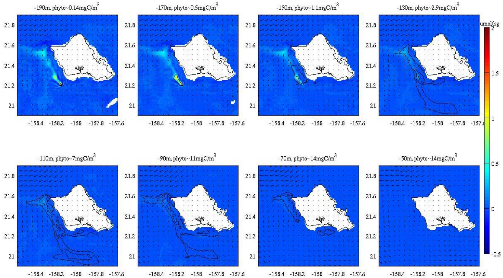
Figure 95. Nitrate perturbation ( \text{umol}/\text{kg} ) due to the RevX 100MW 8x95m OTEC plant, and contour lines of the resultant diatom perturbation (black lines) drawn at intervals of 0.5 \text{ mgC}/\text{m}^3 . June 24 th , 2010 at 16:40 Hawaii Standard Time.
