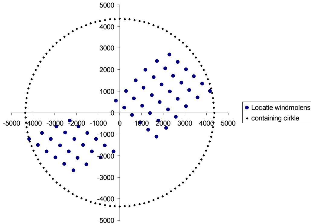
Figure 70. Position of the turbines in the Thorntonbank wind farm with indication of the smallest ‘containing circle’ with radius 4,352m.
